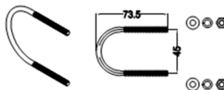
U Bolt
