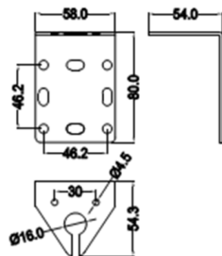
L Bracket
