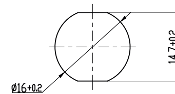
Install size
